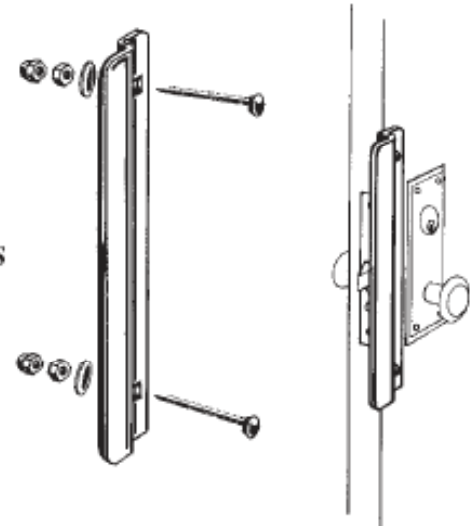
OVDG Offset Guard Plates
